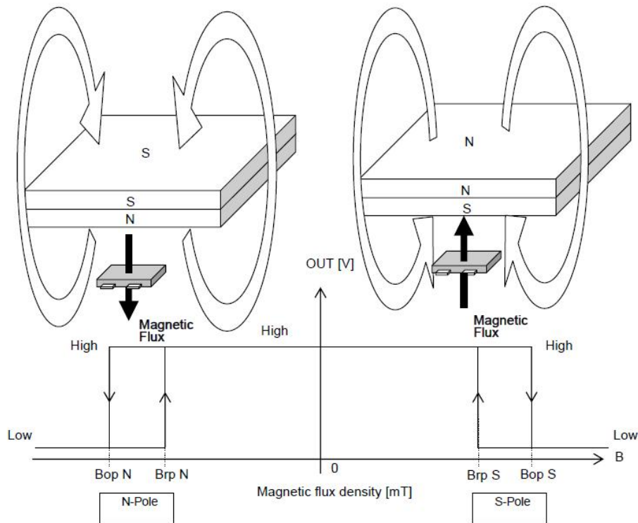
Fig 4, Magnetic Operation Characteristic of AS1803
