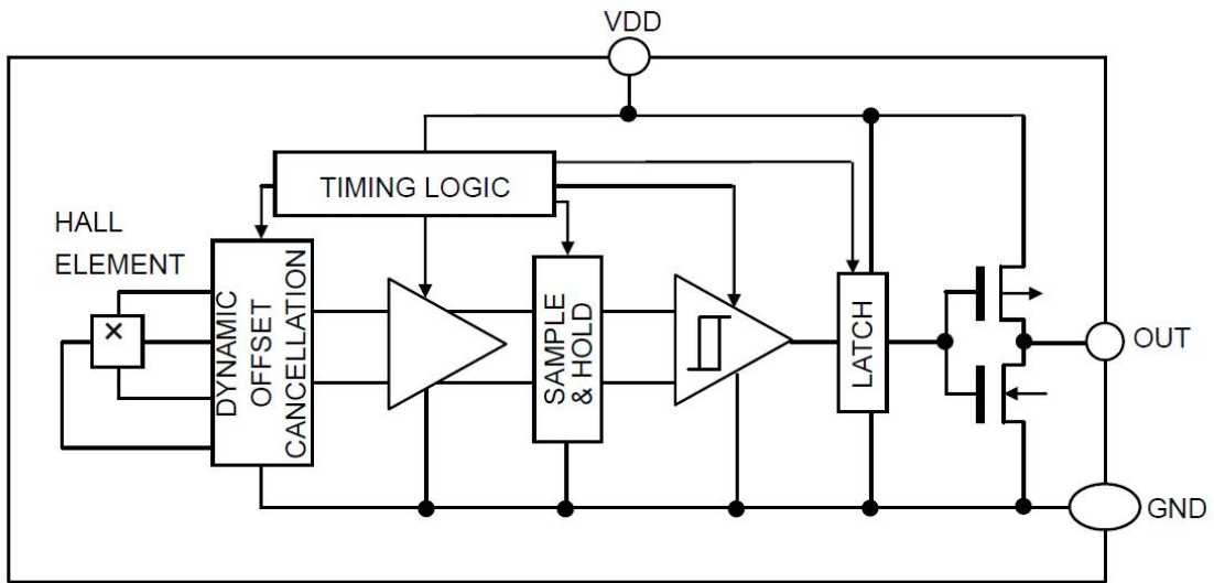
Figure 3, Block Diagram of AS1803
