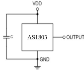
Figure 1, Typical Application Circuit of AS1803
